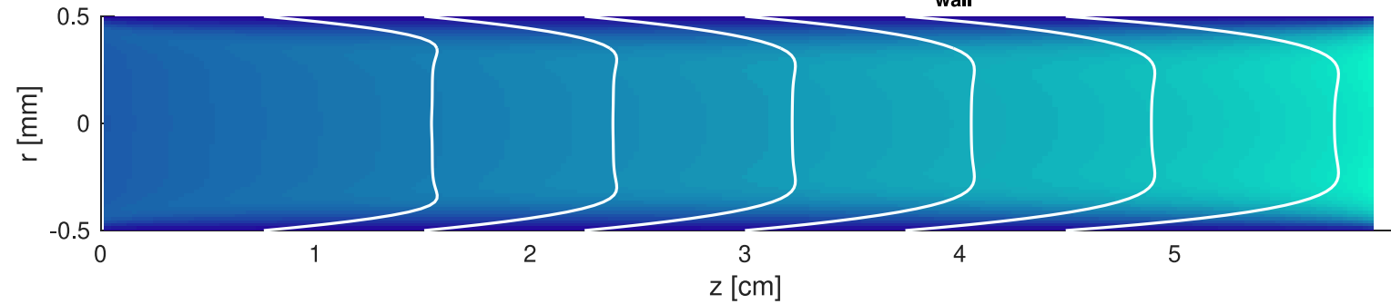
Axial velocity field and radial profiles - T_{\text{wall}} = 500 K
