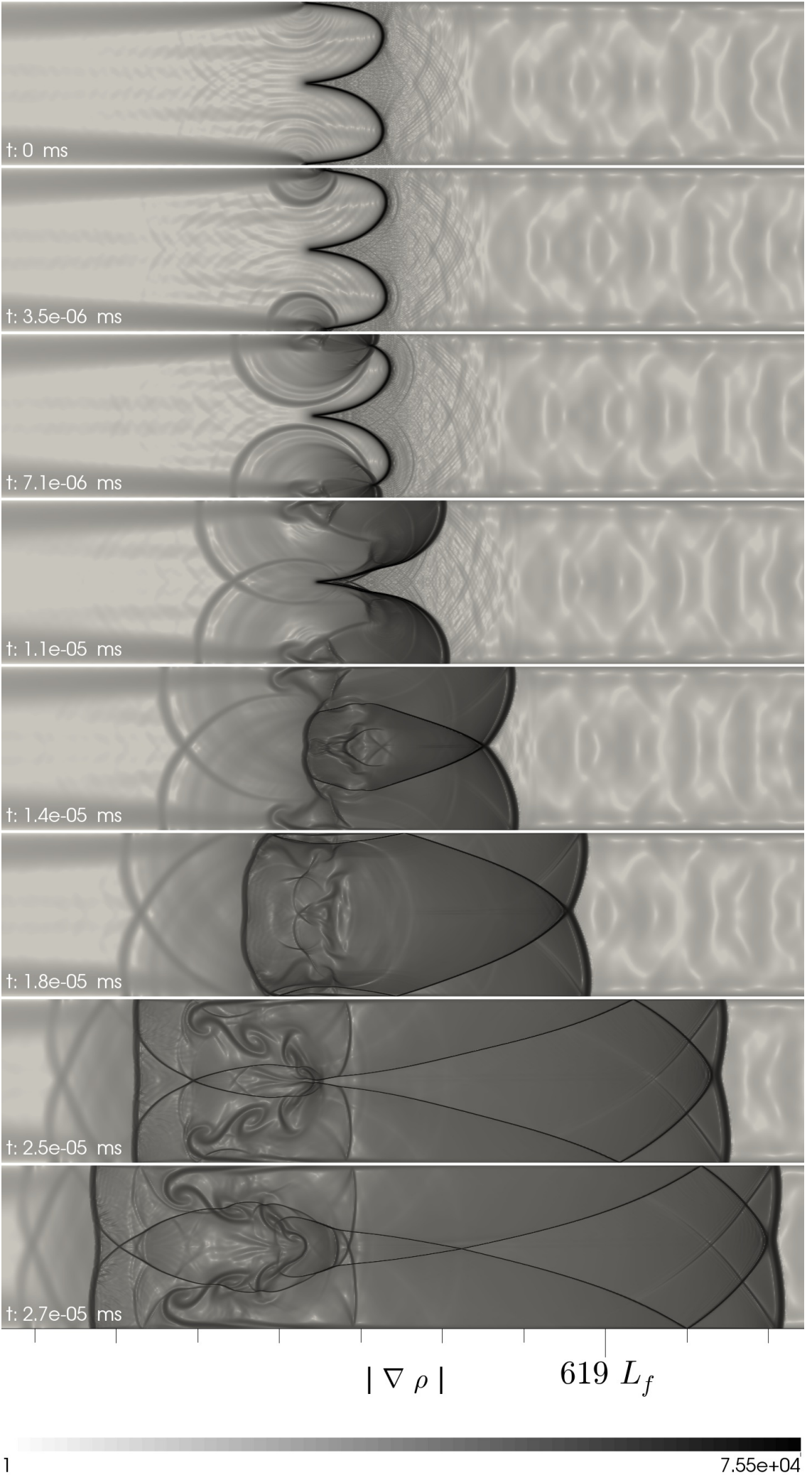
Figure 1: Formation of the preheating zone adjacent to the flame and transition to detonation in a semi-infinite two-dimensional channel with adiabatic no-slip boundaries. The initial conditions are set to a laminar premixed flame of stoichiometric Hydrogen-Air at the left closed end. Calculated with 1024 CPUs.
